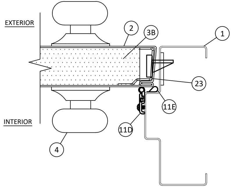
AD 13 HORIZONTAL SECTION AIR INFILTRATION
