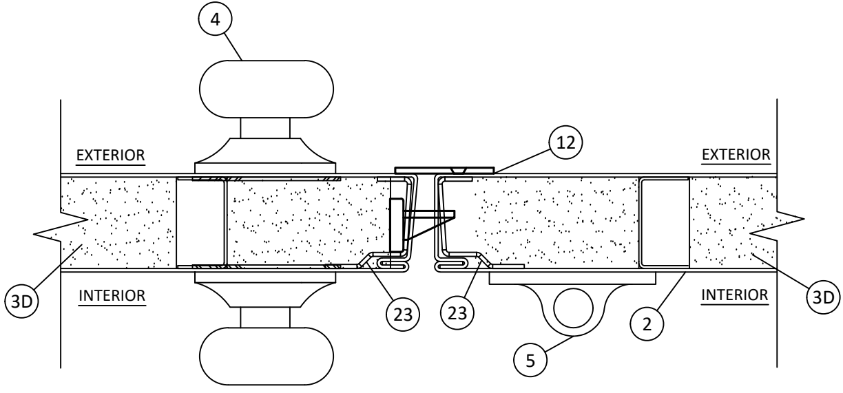
AE 13 HORIZONTAL SECTION AIR INFILTRATION
